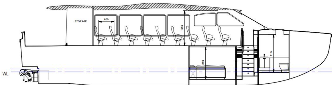
STAR BOARD SECTION Y = -1.760mm
